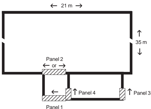
Fig. 9. Diagram of nethouse opening; arrows indicate directions that doors (indicated by slanted boxes) slide
